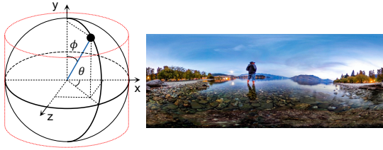
Fig. 11: Equiarectangular projection (ERP) mapping spherical coordinates ( \phi, \theta ) to image pixels ( u, v ), analogous to flattening the Earth onto a world map.
