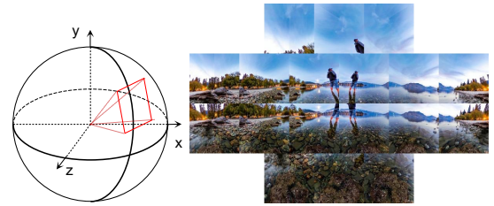
Fig. 13: Tangent projection (TP) maps spherical points onto tangent planes via gnomonic projection, preserving local geometry and enabling perspective model reuse.
